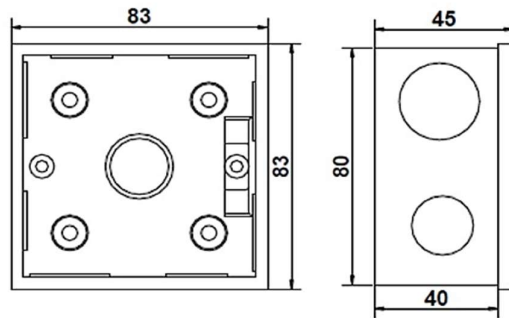
Mounting Box Dimension
